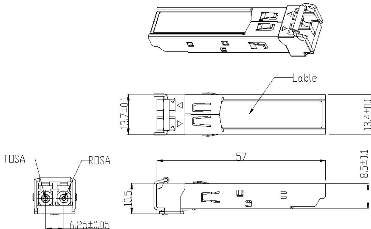
Figure5. Mechanical Dimensions
