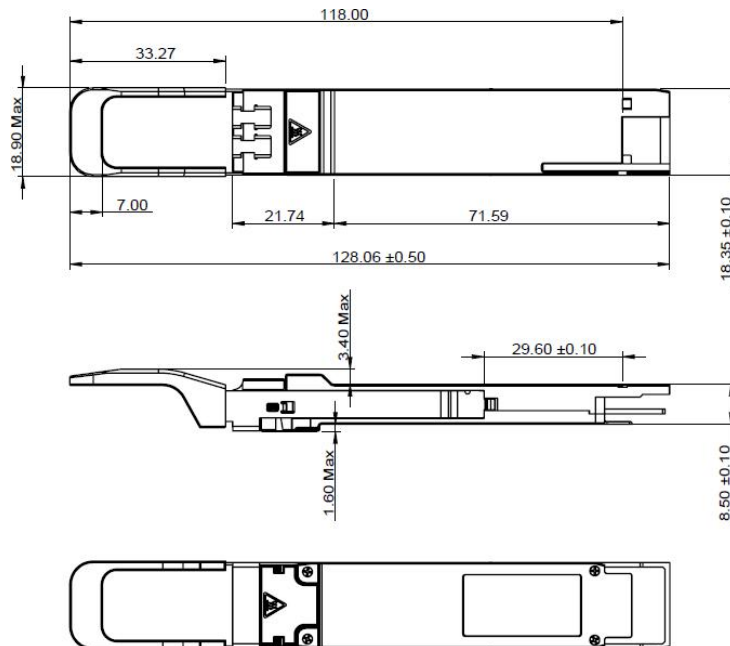
Figure 5. Mechanical Outline
