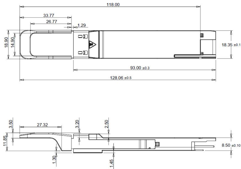
Figure 5. Mechanical Outline
